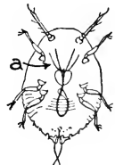
Fig. 373. Beak (a) arising between the fore legs.
